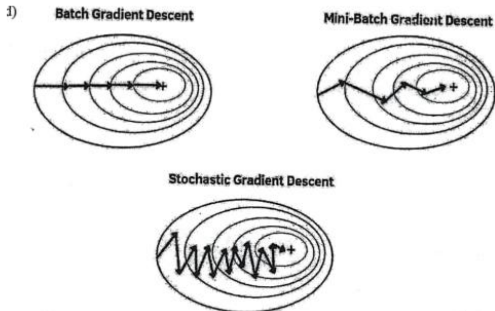
Figure: Optimizers
